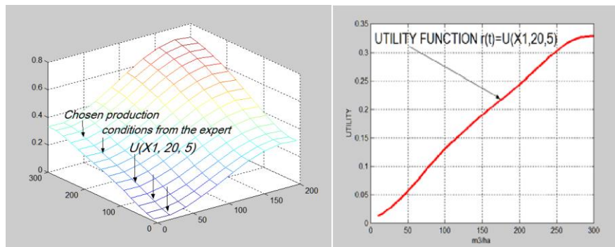
Figure 6. Utility function
