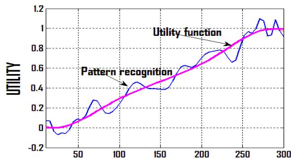
Figure 2. Utility function u(X_1; X_2^o; X_3^o)
