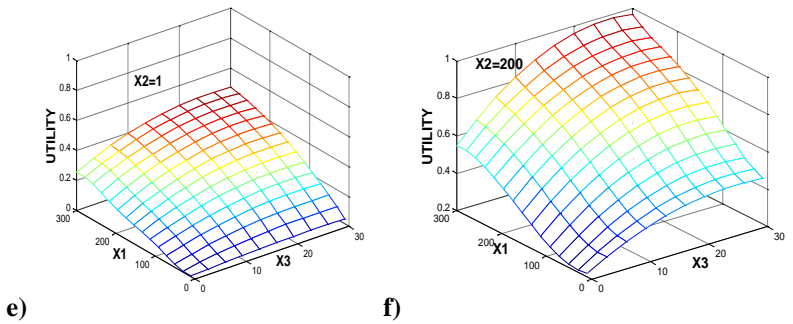
Figure 5. Comparison between utility functions
