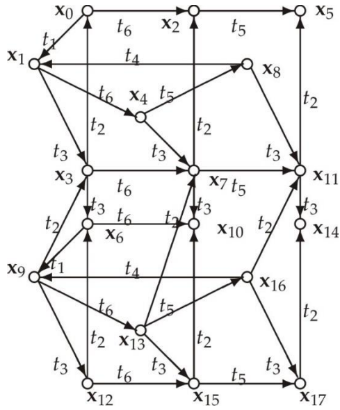
Figure 4. The RG of PN model of the supervised agents
