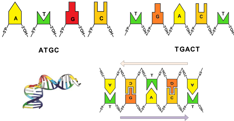
Fig.2. The computer model of DNA.
