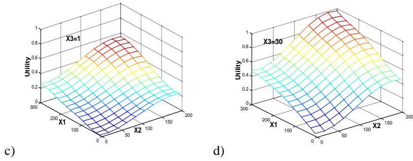
Figure 4. Comparison between utility functions
