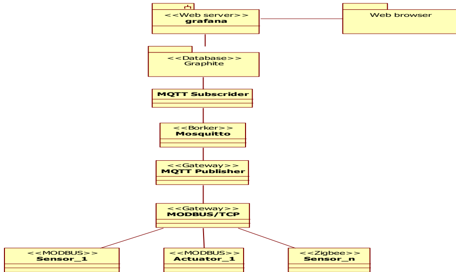
Figure 11. Multi-tier architecture for data collection and management of IoT devices
