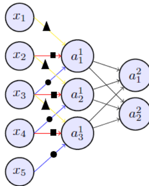
Figure 2. Example of convolutional neural network [8].
