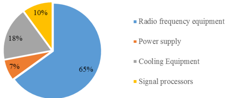
Figure 3. Breakdown of energy consumption of a typical base station with cooling [2].
